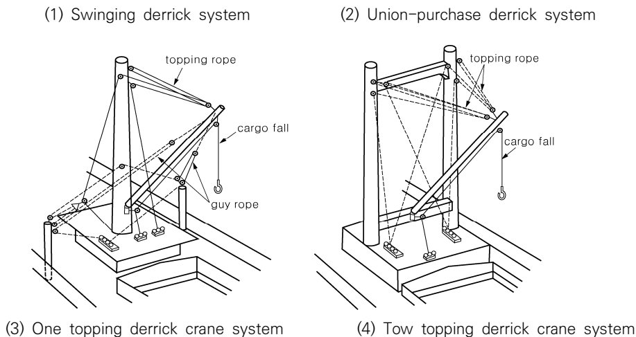
Fig 9.2.1 Derrick Systems
