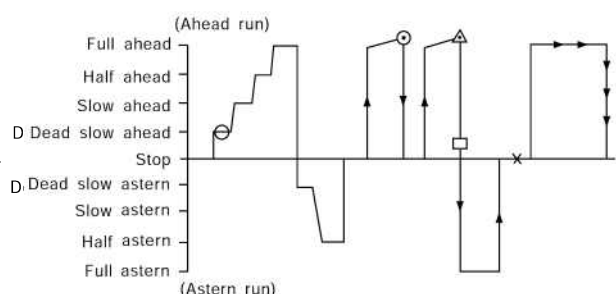
Fig 9.3.2 Trial Procedures for Steam Turbines Ships (2021)
